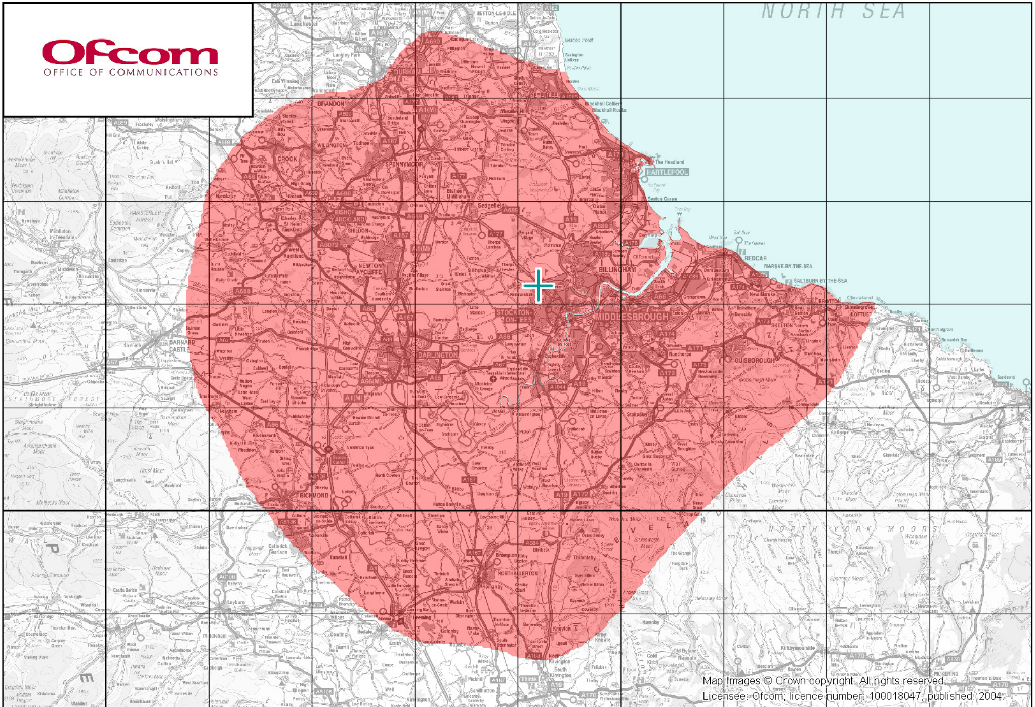
Teesside AM MCA (Magic 1170) - 29th December 2003
