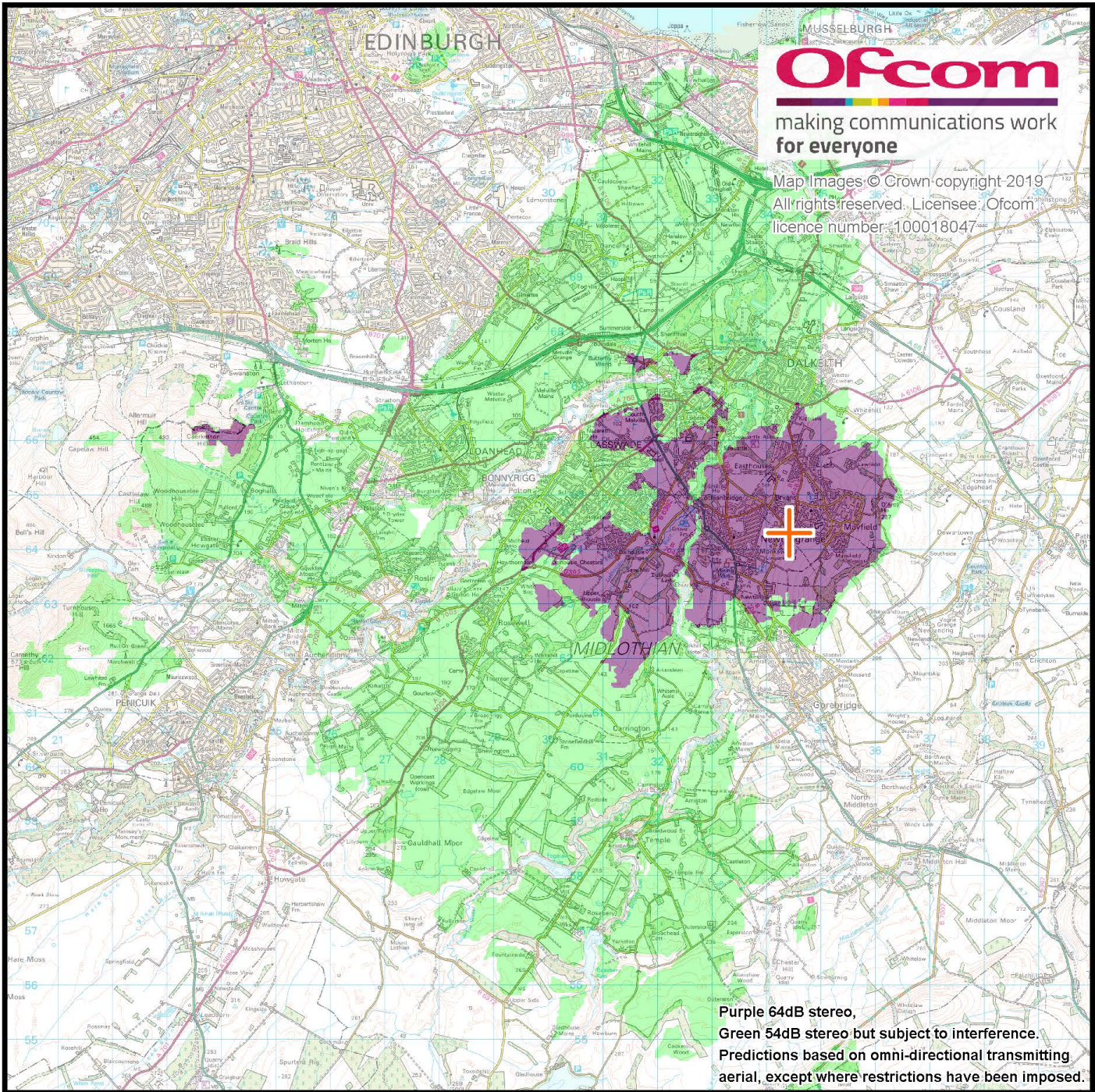
Newtongrange (Black Diamond) community radio coverage area - 8th November 2018
