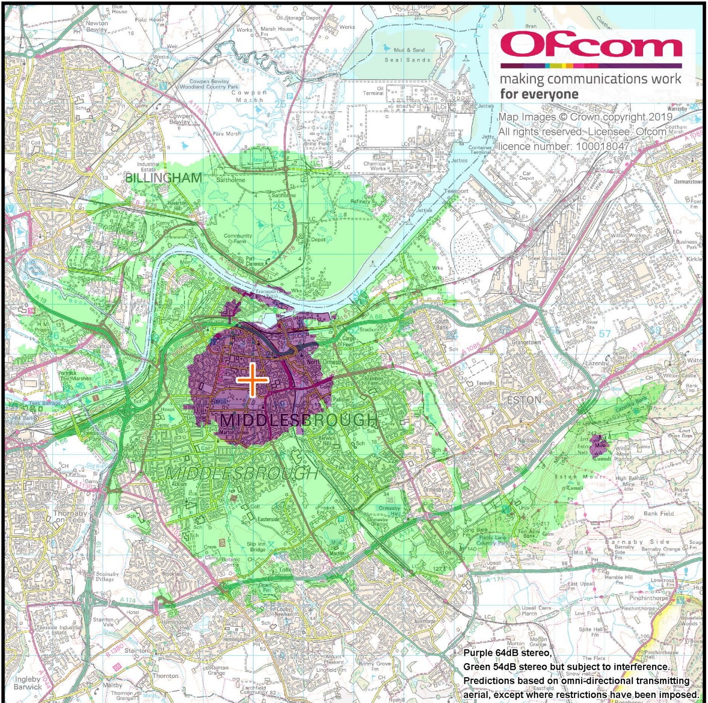
Middlesbrough (Community Voice FM) community radio coverage area - 15th April 2014
