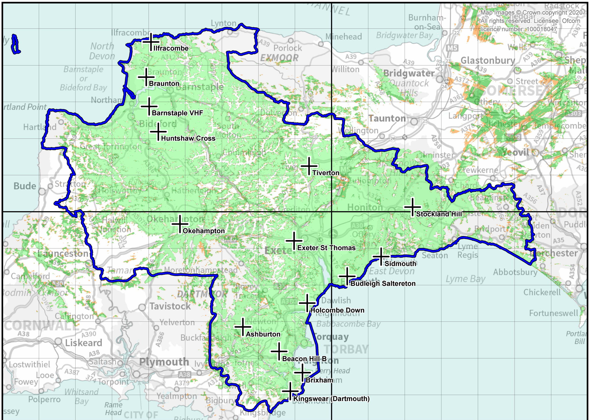
Exeter & Torbay/North Devon local DAB Multiplex service (NOW Digital) Indoor coverage, enhanced propagation conditions, August 2020
