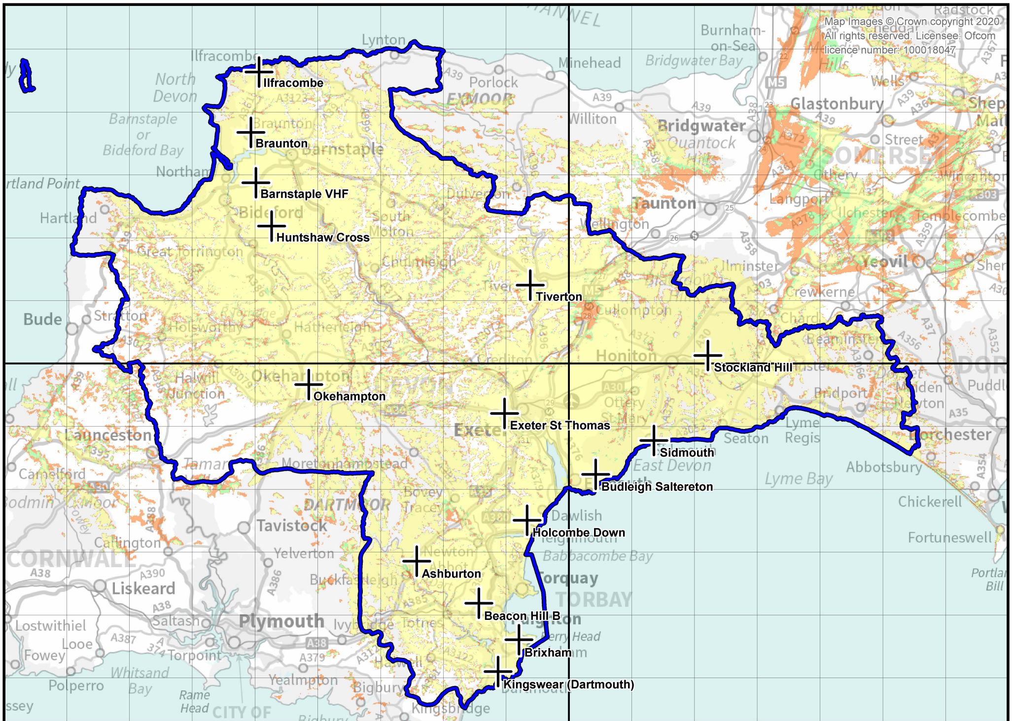
Exeter & Torbay/North Devon local DAB Multiplex service (NOW Digital) Mobile coverage, enhanced propagation conditions, August 2020
