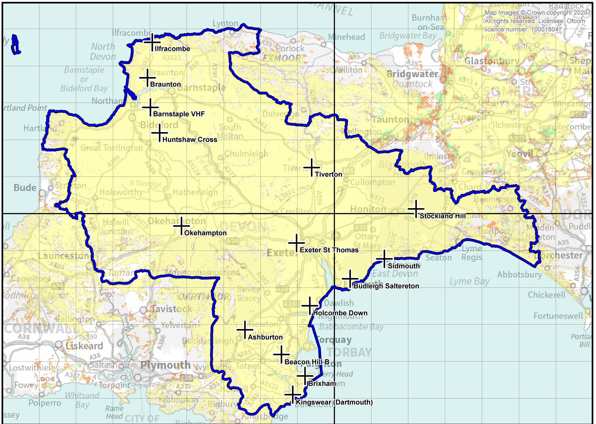
Exeter & Torbay/North Devon local DAB Multiplex service (NOW Digital) Mobile coverage, normal propagation conditions, August 2020
