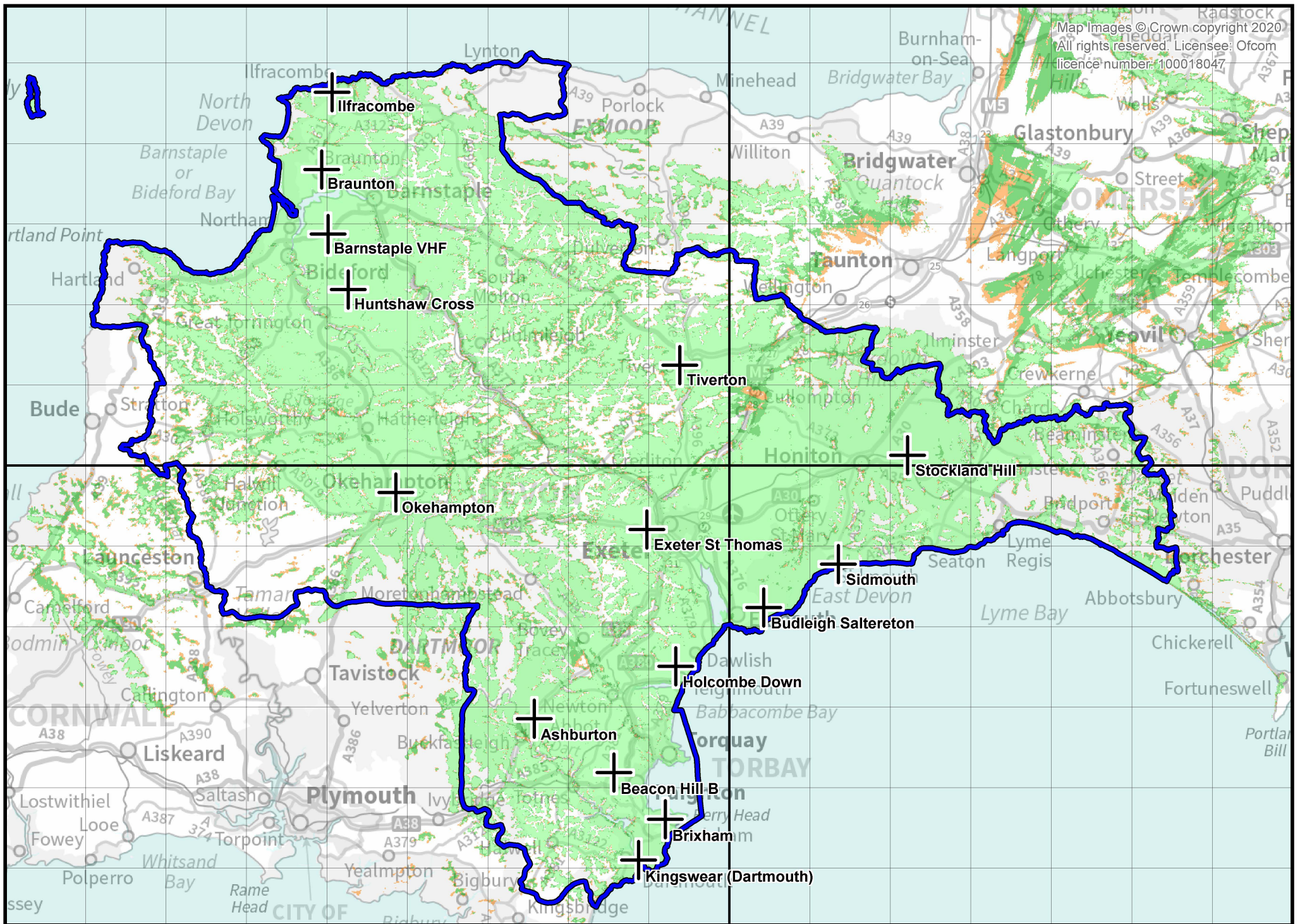
Exeter & Torbay/North Devon local DAB Multiplex service (NOW Digital) Indoor coverage, normal propagation conditions, August 2020
