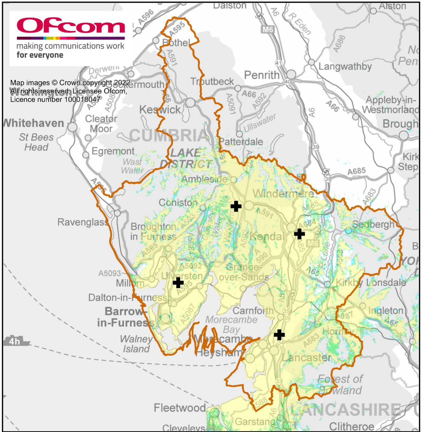
Morecambe Bay local DAB multiplex service (MuxCo). Mobile coverage, normal propagation conditions. May 2022.
