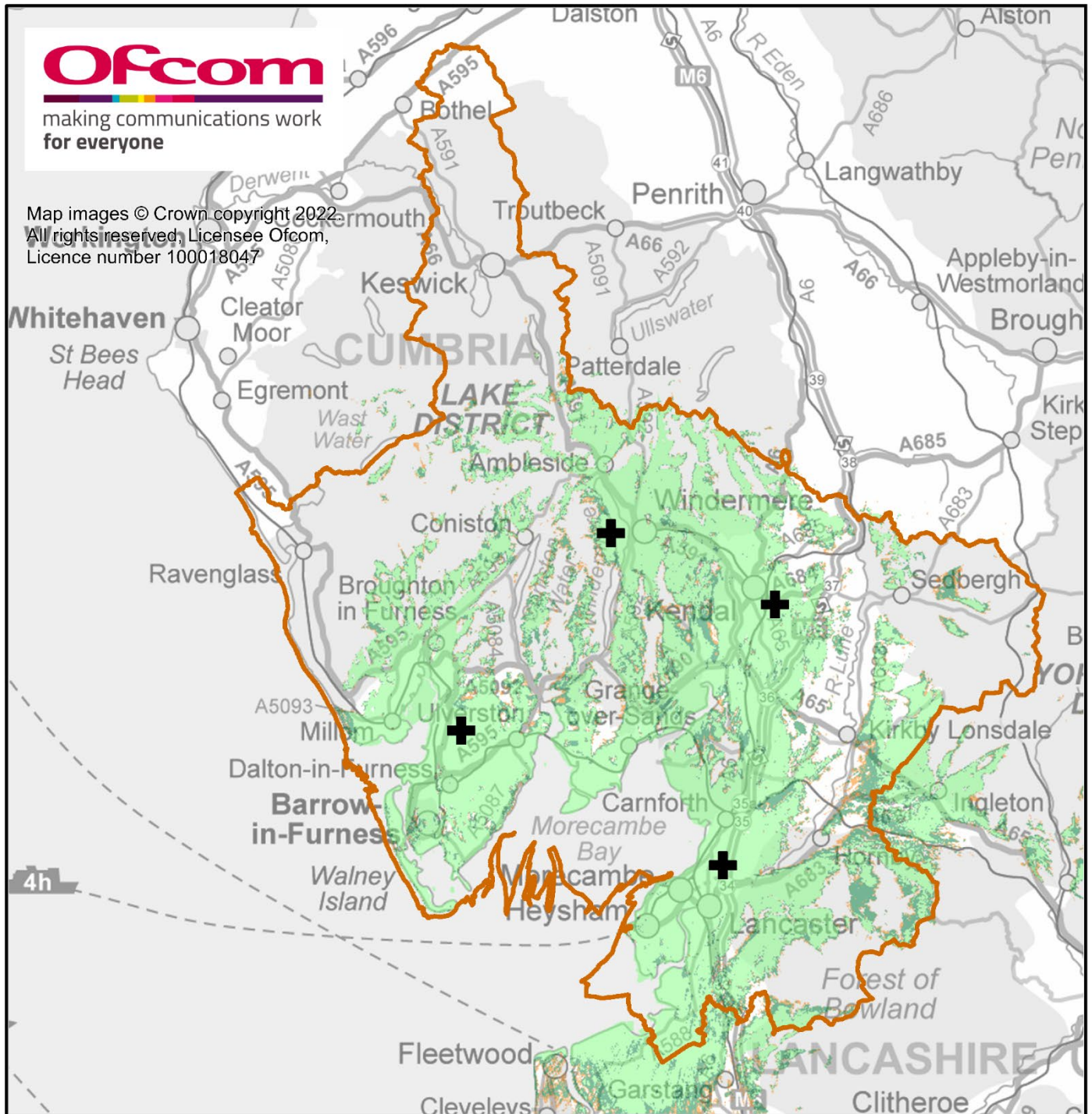
Morecambe Bay local DAB multiplex service (MuxCo). Indoor coverage, normal propagation conditions. May 2022.
