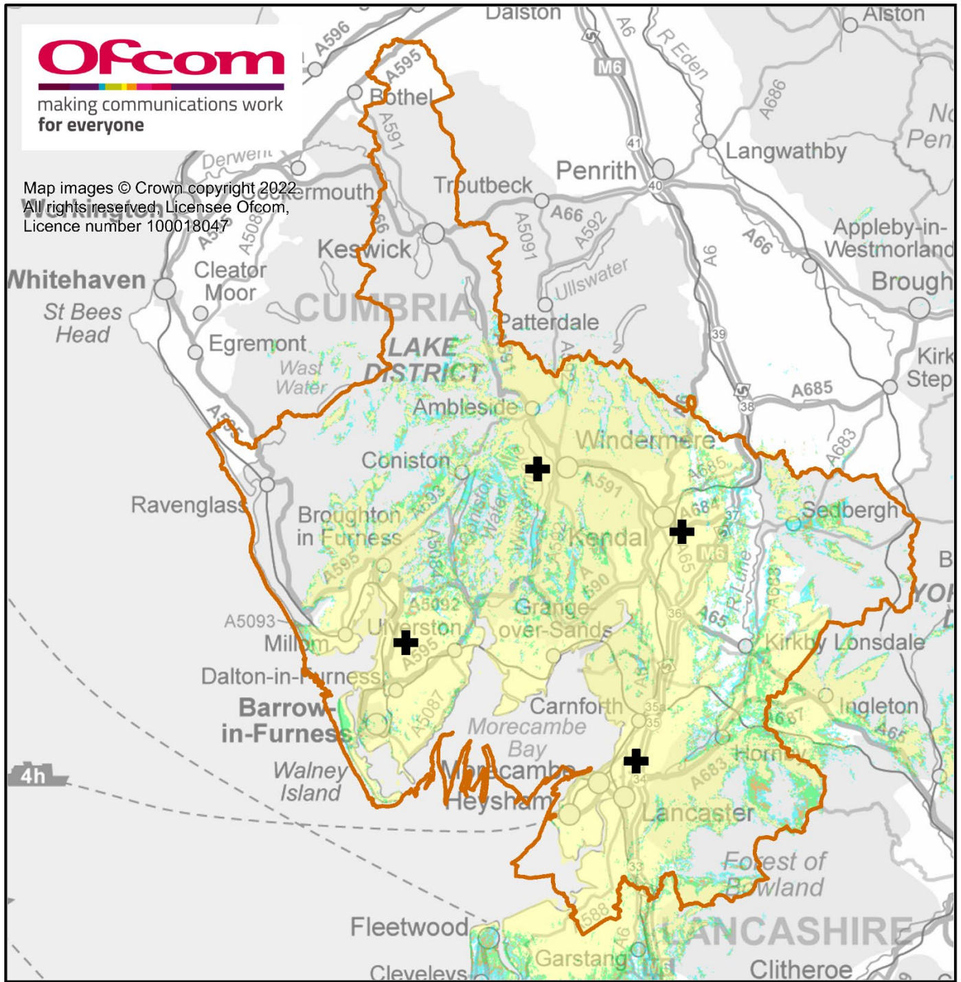
Morecambe Bay local DAB multiplex service (MuxCo). Mobile coverage, enhanced propagation conditions. May 2022.
