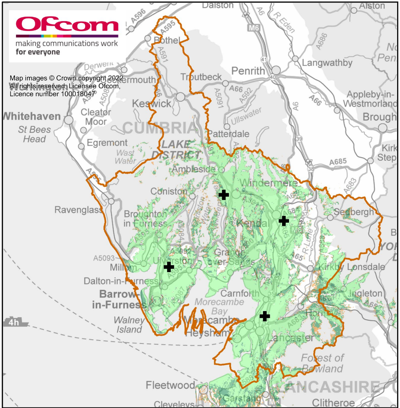
Morecambe Bay local DAB multiplex service (MuxCo). Indoor coverage, enhanced propagation conditions. May 2022.
